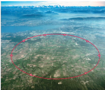
Figure 44.7 (a) The Large Hadron Collider at the European Organization for Nuclear Research (CERN). The underground accelerating ring (shown by the red circle) is 100 m underground and 8.5 km in diameter, so large that it spans the border between Switzerland and France. (Note the Alps in the background.) When accelerated to 7 TeV, protons travel around the ring more than 11,000 times per second. (b) An engineer working on one of the 9593 superconducting electromagnets around the LHC ring.
