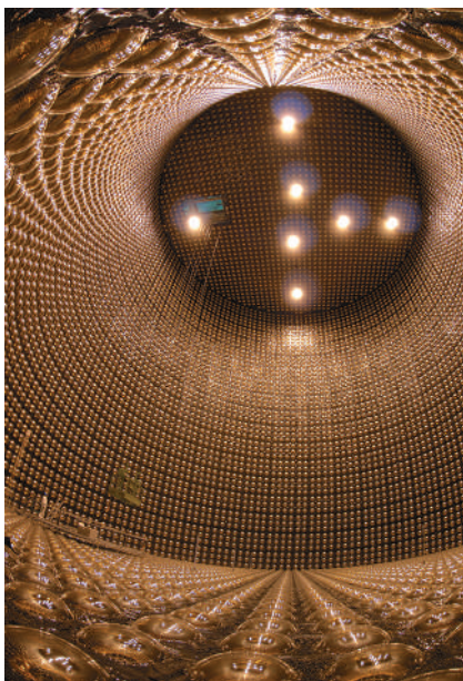
Figure 44.15 This photo shows the interior of the Super-Kamiokande neutrino detector in Japan. When in operation, the detector is filled with 5 \times 10^7 kg of water. A neutrino passing through the detector can produce a faint flash of light, which is detected by the 13,000 photomultiplier tubes lining the detector walls. Data from this detector were the first to indicate that neutrinos have mass.
